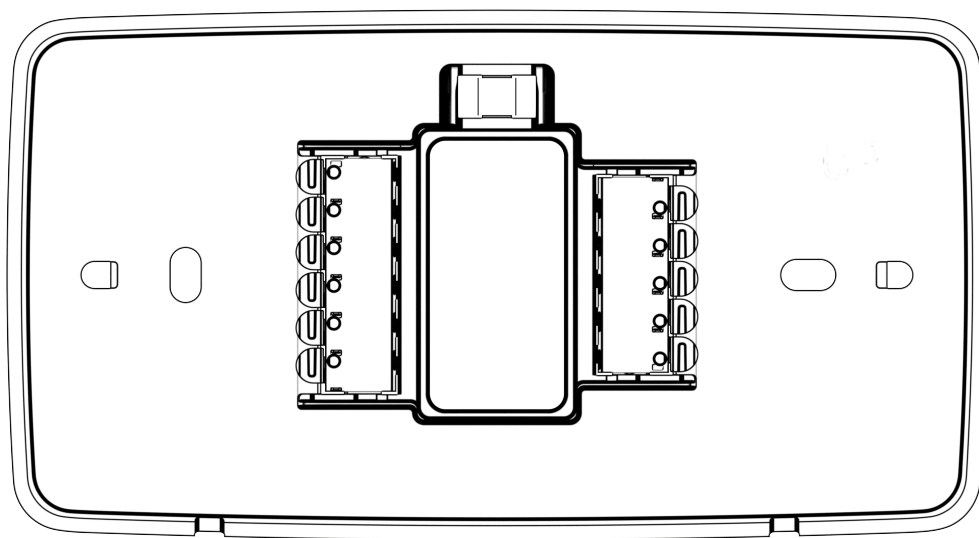
Thermostat backplate
